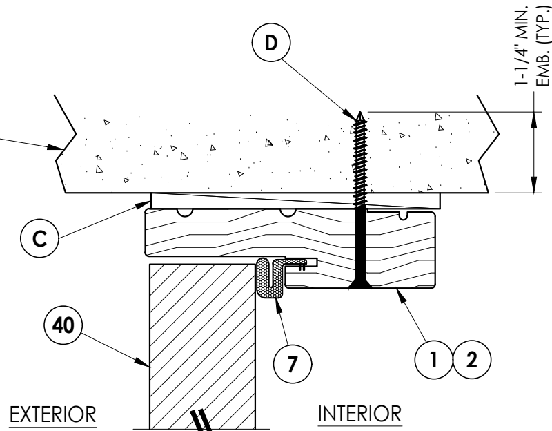
3 7 VERTICAL CROSS SECTION Shown Direct to Masonry Outswing shown (Inswing similar)
